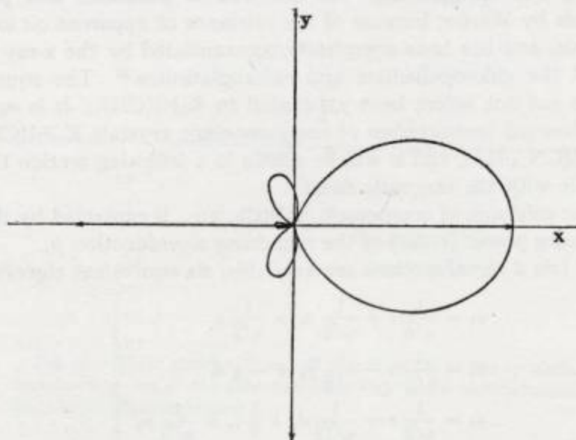
Fig. 9.—Polar graph of \left| \frac{1}{2} + \frac{\sqrt{3}}{2} \cos \varphi + \frac{\sqrt{15}}{4} \cos 2 \varphi \right| in the xy plane, representing one of the four equivalent dsp^3 bond eigenfunctions. The directions of the maxima of the four are represented by arrows.
