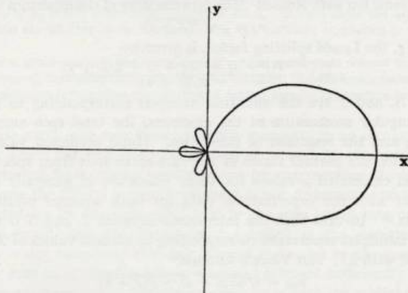
Fig. 10.—Polar graph of |\psi_1| of Equation 13, in the xy plane, representing one of the six equivalent d^2sp^3 bond eigenfunctions (octahedral eigenfunctions).
