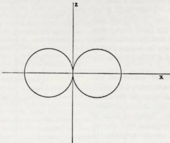
Fig. 2.—Polar graph of |\sqrt{3} \sin \theta| in the xs plane, representing the p_x eigenfunction.
